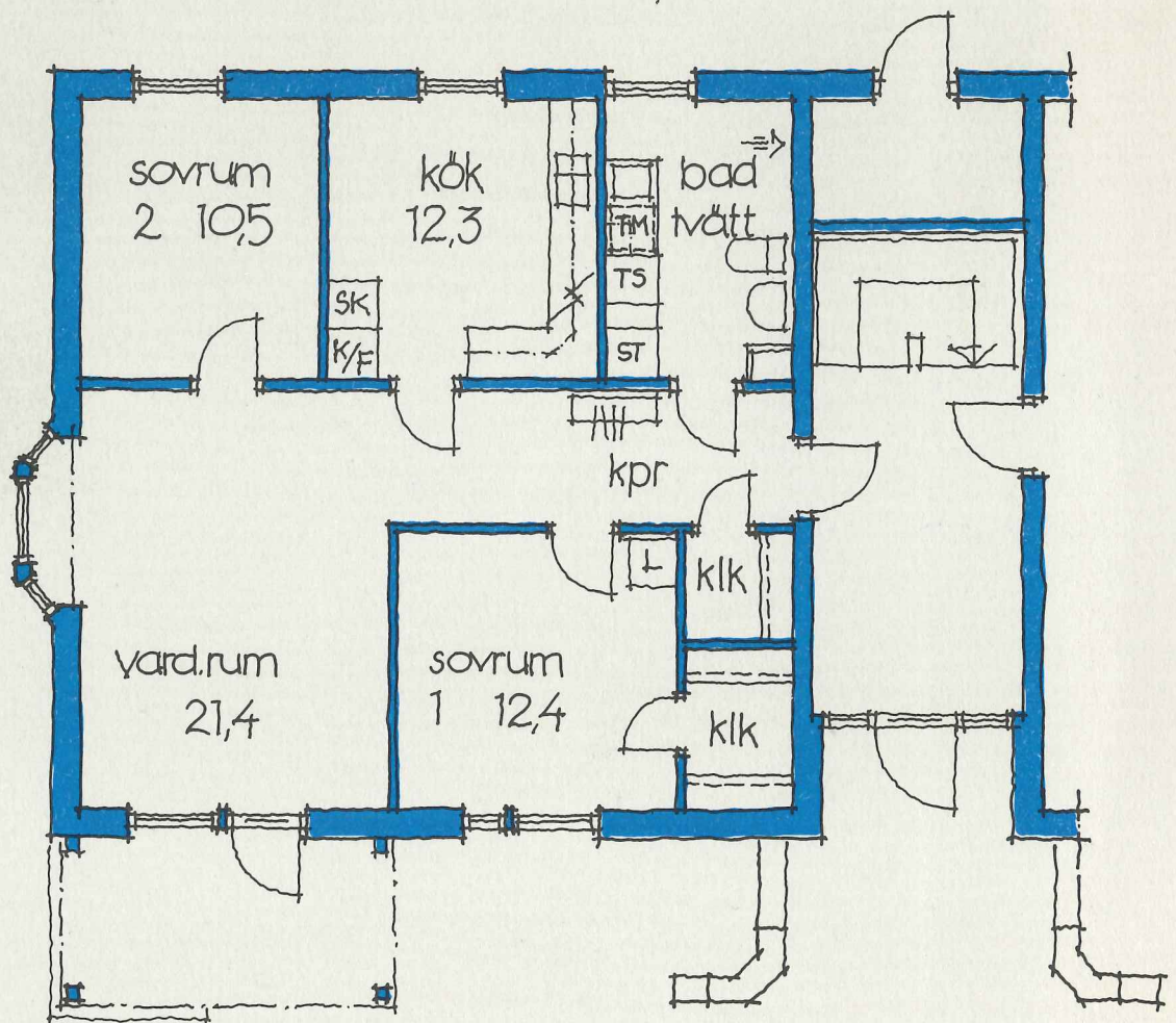
bottenplan
